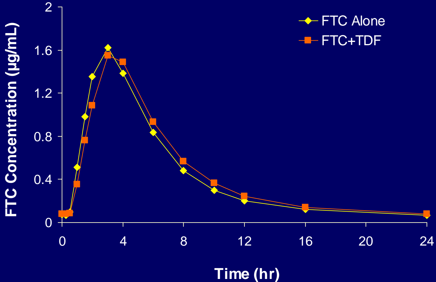
Figure 1. Mean FTC Plasma Concentration-time Profiles
